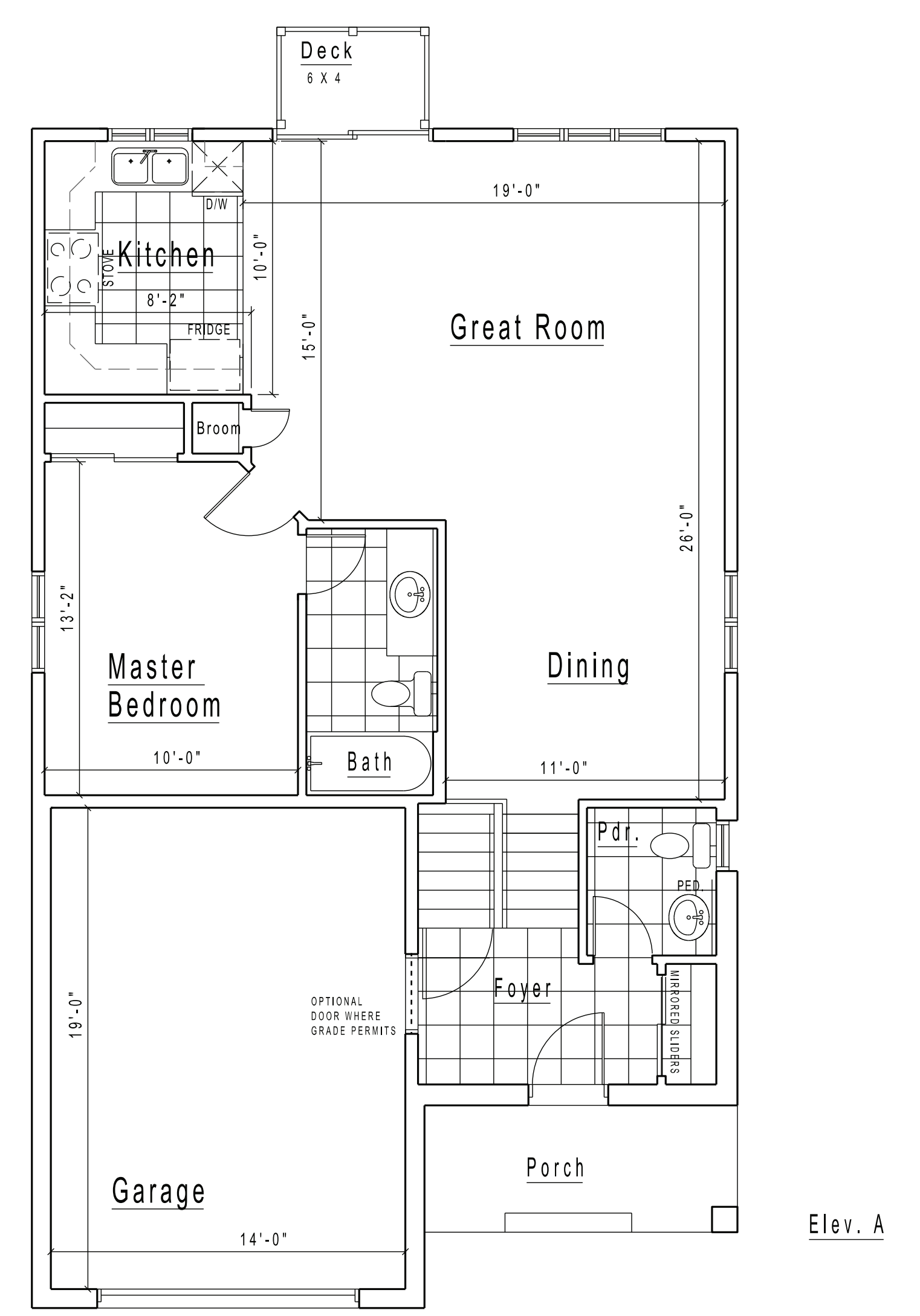
Ground Floor 900 s.f.
