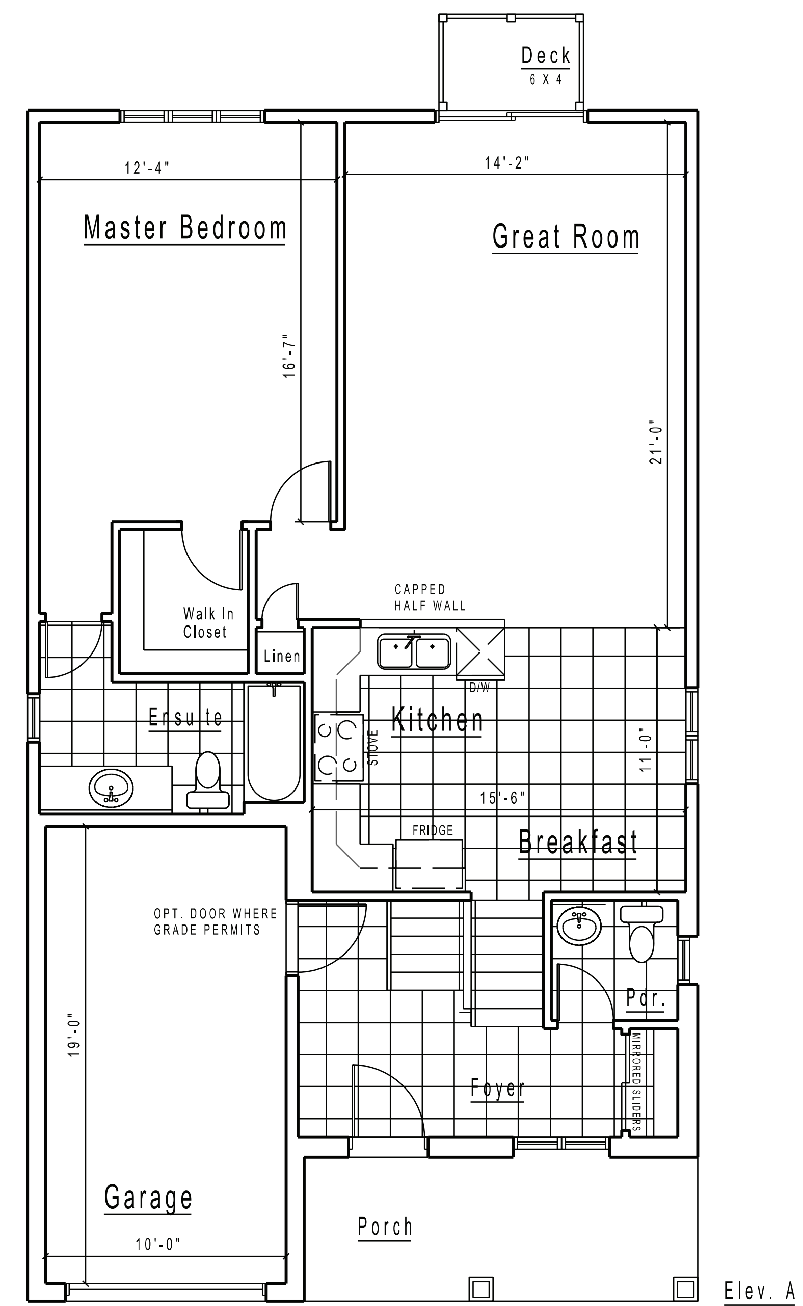
Ground Floor
