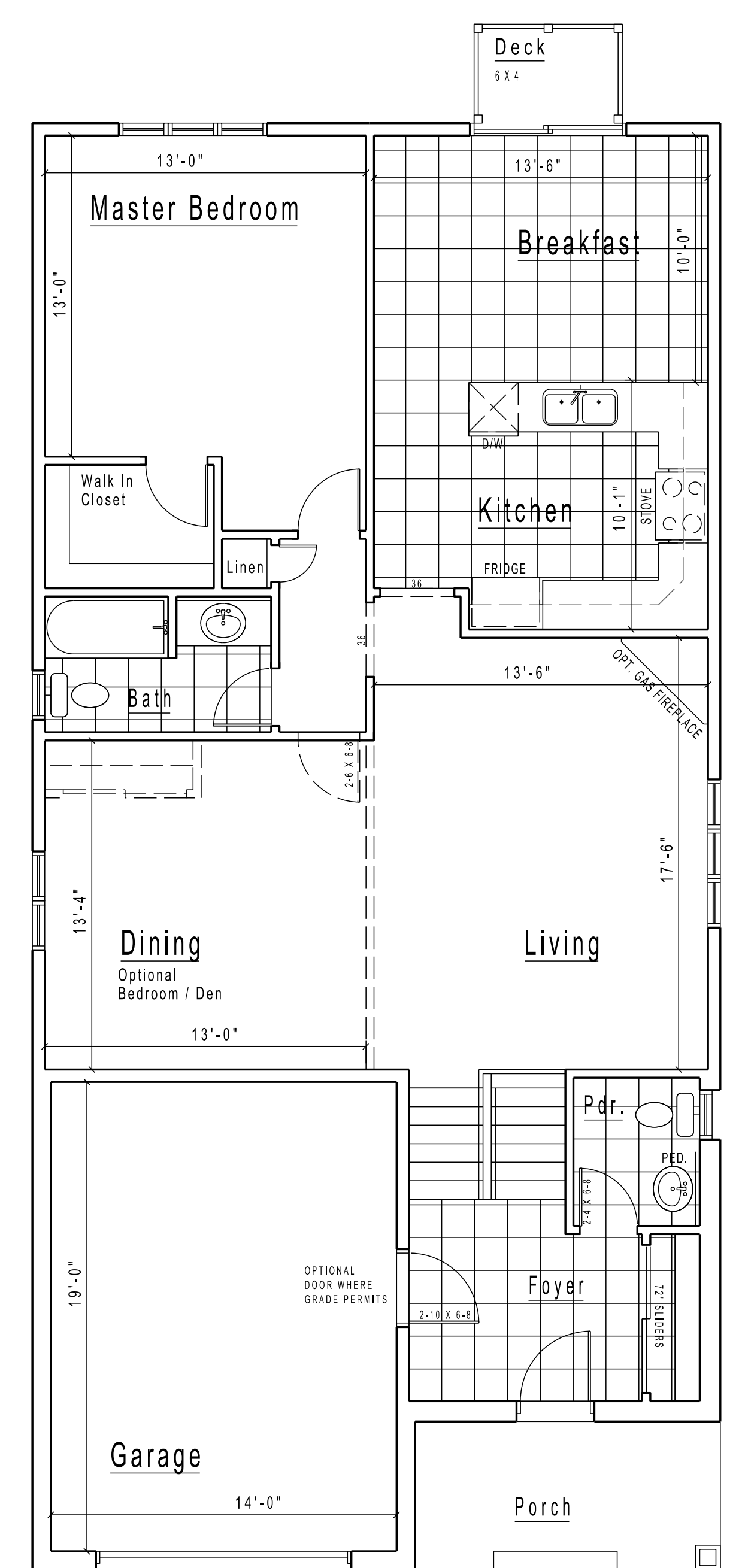
Ground Floor Opt. 1260 s. f.
